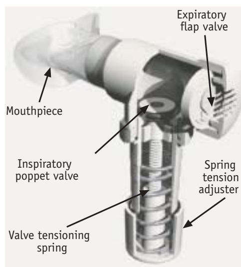
Figure 1 An exploded view of the internal construction of a mechanical pressure threshold training device.
